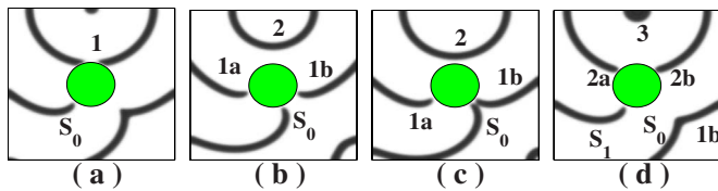
FIG. 1. (Color online) (a) Wave S_0 , pinned to an obstacle (shaded), rotates counterclockwise; wave 1 is the first pacing wave. (b) Wave 1 hits the obstacle and separates into a wave rotating counterclockwise (1a) and a wave rotating clockwise (1b). (c) Waves S_0 and 1b collide and merge leaving only one rotating wave 1a denoted S_1 hereafter. (d) The wave resulting from the merging of S_0 and 1b leaves the system. The interaction between the following pacing wave, 2 and S_1 , is similar to that shown in (a)–(c). Thus, the pinned vortex persists. Numerical simulation of the Barkley model with parameters: a=0.9 , b=0.17 ; the pacing period is T_p=6.7 and the radius of the obstacle is R=6.5 .
