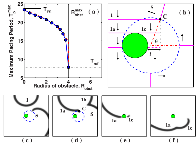
FIG. 4. (Color online) (a) The maximum pacing period T_p^{max} at which unpinning is possible as a function of the obstacle radius R_{obst} . For the parameters a = 1.1323 , b = 0.2459 that we have used, the maximum radius of obstacle from which depinning can occur is R_{obst}^{max} = 4 . T_{FS} is the period of a free spiral wave and T_{ref} is the refractory period. The dashed line indicates the prediction from Eq. (2). (b) The wavelet formation mechanism leading to the detachment of the pinned vortex (schematic). (c)–(f) Numerical simulation of the Barkley model. S collides with wave 1 at point C at an angle \theta . The part 1b of the pacing wave merges with S , moving out of the system. The remaining part of the pacing wave collides with the obstacle (shaded) separating into 1a and a small wavelet 1c . When the length l of wavelet 1c is larger than the critical nucleation length, 1c survives and collides with S . This results in unpinning of S .
