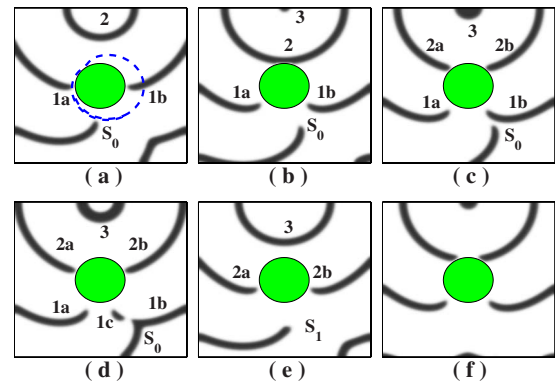
FIG. 2. (Color online) Lowering excitability results in successful detachment of pinned vortex by pacing. S_0 is a rotating wave whose core (dashed line) is larger than the pinning center (shaded). (a)–(c) are topologically as in Fig. 1. (d) A wavelet 1c is produced after collision of waves S_0 and 1b in contrast with Fig. 1(d). (e) The wavelet 1c collides with 1a and the resulting wave S_1 is displaced away from the obstacle. (f) Subsequent pacing induces drift of the spiral wave S_1 to the boundary eventually removing it from the medium. The parameters are as in Fig. 1, except for a=0.895 and b=0.1725 , resulting in increasing the vortex core size.
