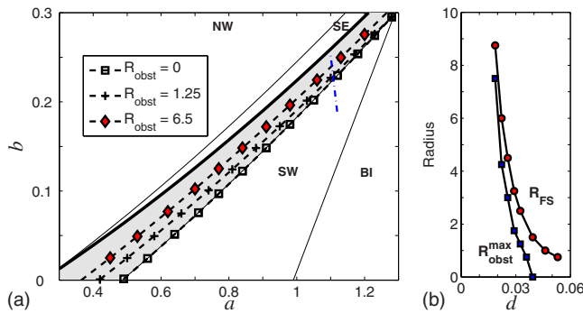
FIG. 3. (Color online) (a) Parameter space of the Barkley model. Unpinning is possible in the shaded portion of the SW region, which exhibits persistent spiral waves. The thick line indicates the boundary with the SE region, where spirals cannot form. The domain where unpinning is possible shrinks with increasing size of the pinning center, the three dashed lines corresponding to R_{obst} = 0 , i.e., no obstacle, R_{obst} = 1.25 (plus), and R_{obst} = 6.5 (diamond). (b) Radius R_{FS} of the free spiral and the maximum obstacle radius R_{obst}^{max} from which wave trains can unpin vortices, as a function of the distance d from the SE-SW boundary, along the dot-dashed line indicated in (a). Note that R_{FS} > R_{obst}^{max} and both increase with decreasing d . [In (a), NW (BI) indicates the parameters for which steady waves are absent (the medium is bistable).]
